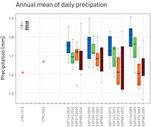
Figure 19. Annual mean of daily precipitation sums for the Thaya basin based on advanced delta-method.
