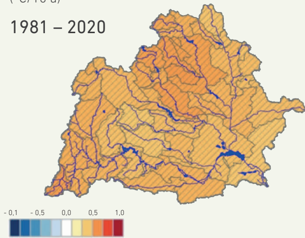
Figure 6. Spatial patterns of trends in annual temperature.
