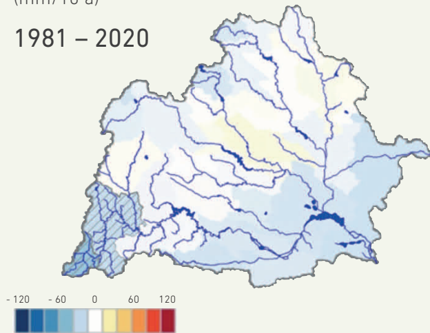
Figure 7. Spatial patterns of trends in annual rainfall.
