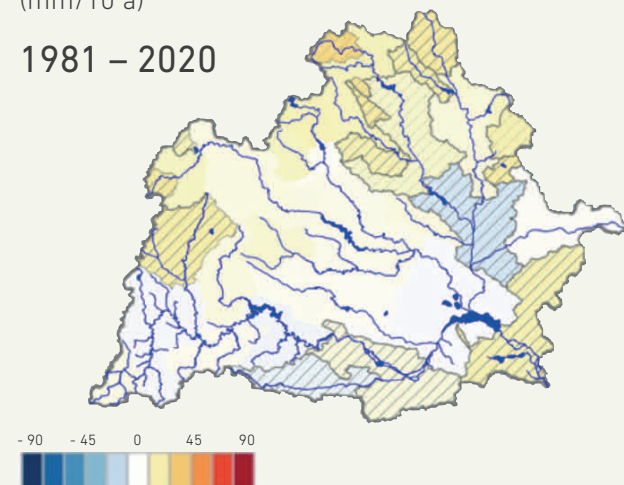
Figure 8. Spatial patterns of trends in annual runoff.
