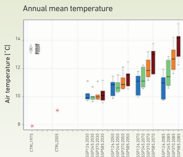
Figure 17. Comparism of air temperature in different climate models.
